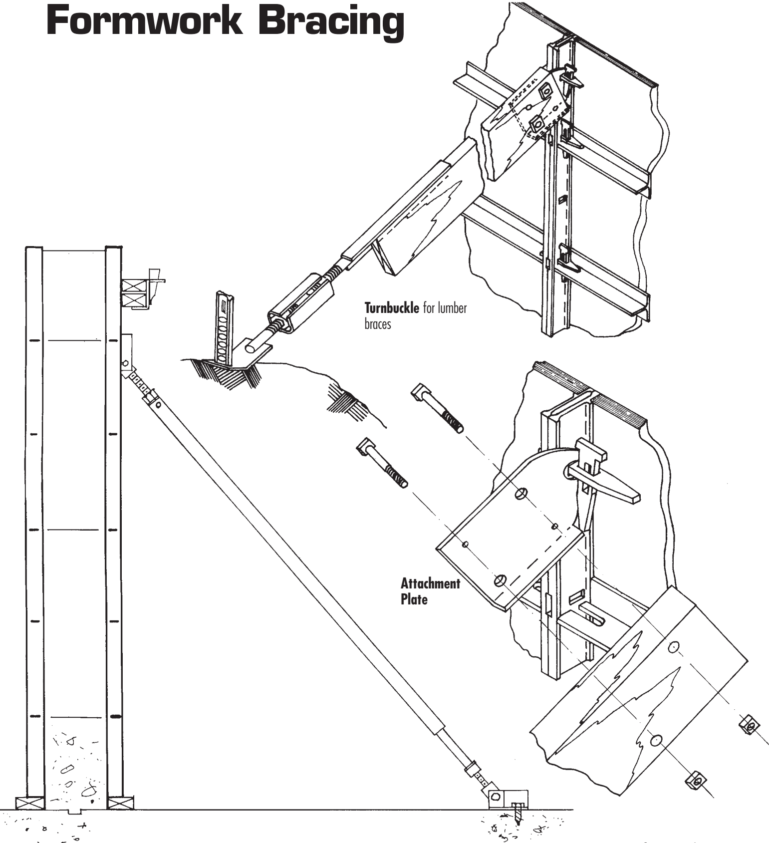
Pipe Brace utilization.
