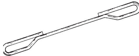
Stiff Back Tie Similar to the Waler Tie, it is used for Vertical Stiff Backs behind the Walers.
