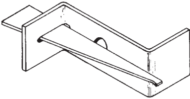
Z Tie Holder This attaches double Walers and stiff backs to Modular Form Panels with the use of a Waler Tie.
